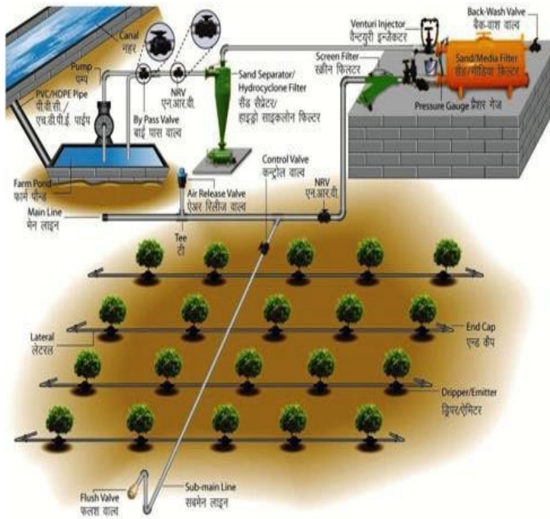
Fig.7.1.Component and layout of drip irrigation system.
