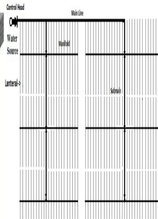
Fig.7.2.Typical layout of drip irrigation system.
