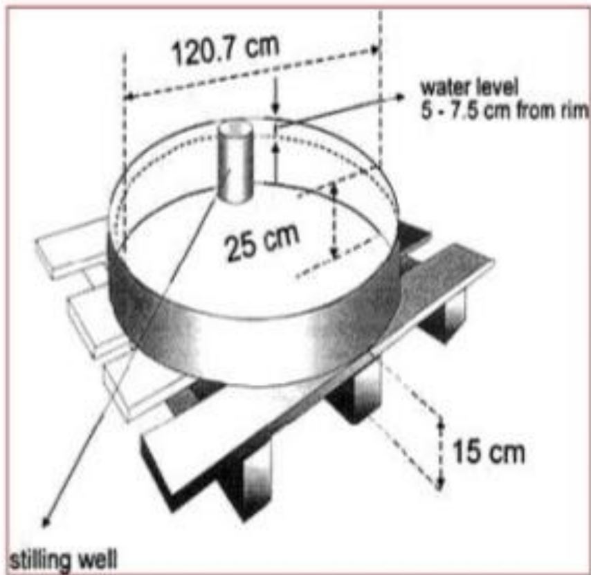
Fig. 19.2. USWB Class A Pan evaporimeter
