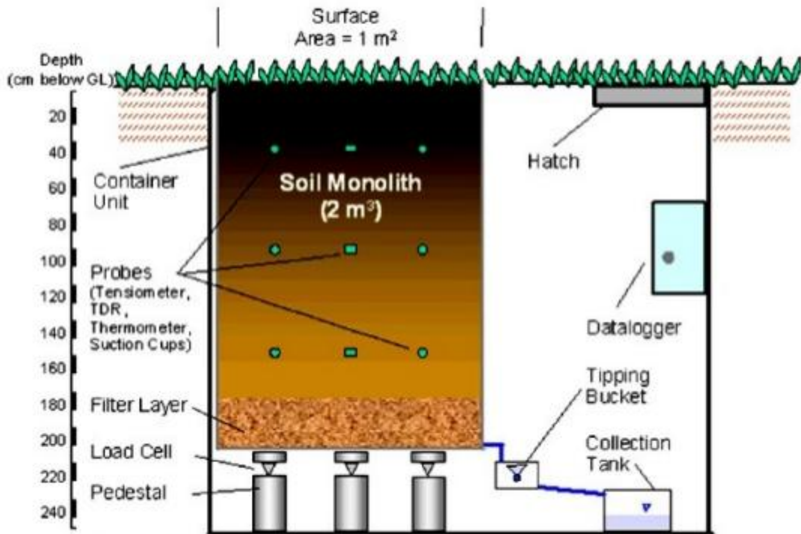
Fig. 19.1. schematic view of Lysimeter
